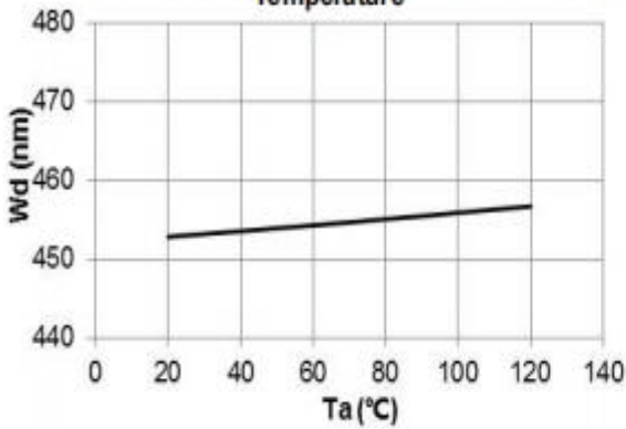
Fig.5-Dominant Wavelength (@120mA) vs. Ambient Temperature
