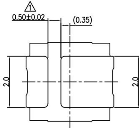
建议焊盘尺寸图 Recommended Soldering Pattern
