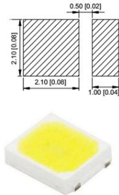
建议焊盘尺寸图 Recommended Soldering Pattern
