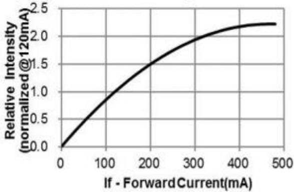
Fig.1-Relative Luminous Intensity vs. Forward Current
