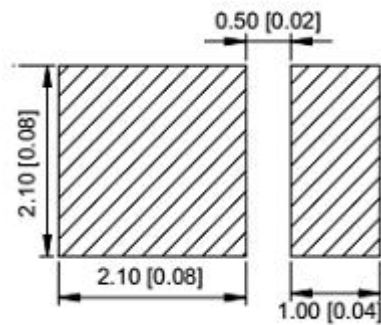
建议焊盘尺寸图 Recommended Soldering Pattern
